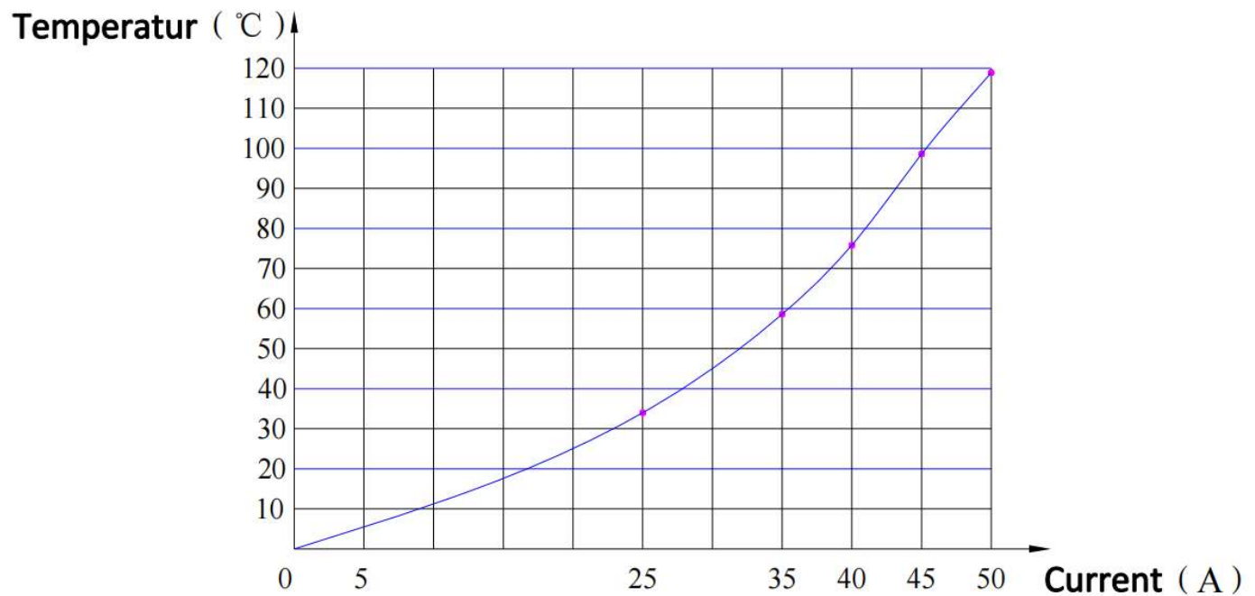
Figure 6.1 Contact Temperature Rise vs Current Curve
